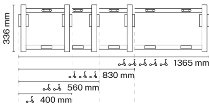
SB 1 - wall
